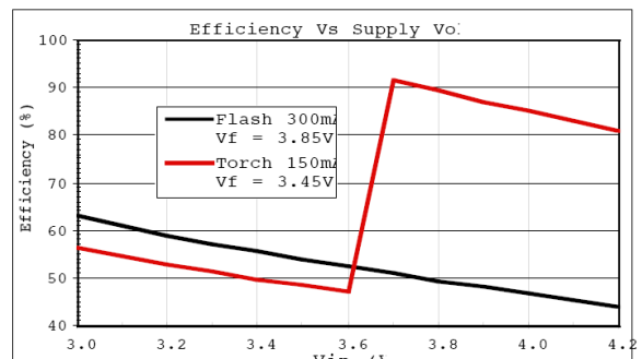
Fig. 15: Efficiency vs Supply Voltage D1=AOT3228HPW0303B LED, R SENSE =0.3Ω R SET =140kΩ, C IN =2.2μF, C FC =0.47μF, C OUT =1μF
