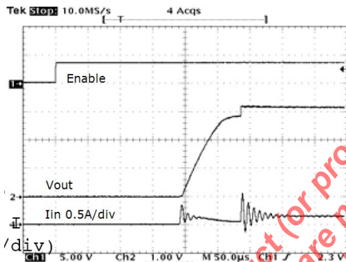
Fig. 18: Startup Torch V_{IN}=3.6V , V_{OUT}=3.1V , C_{IN}=4.7\mu F , C_{FC}=0.47\mu F , C_{OUT}=2.2\mu F
