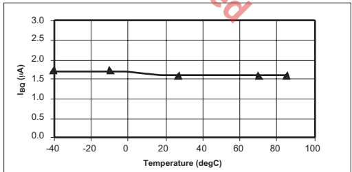
Figure 16. I_{batq} Pin Quiescent Current vs. Temperature, ( V_{out}=3.3\text{V} ), V_{batt}=1.0\text{V}
