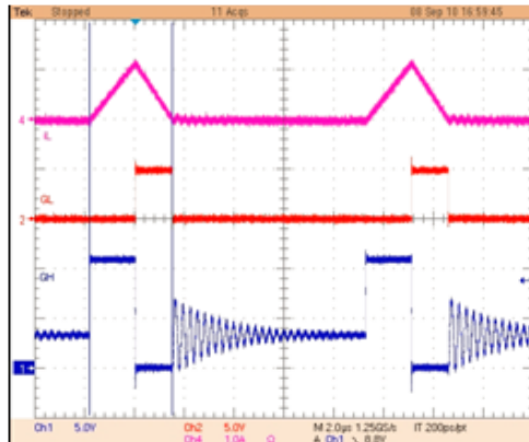
Figure 5: PFM Zero Current Accuracy
