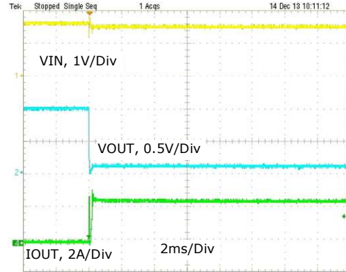
Fig. 5: Short-circuit, 1.5VIN, 1VOUT
