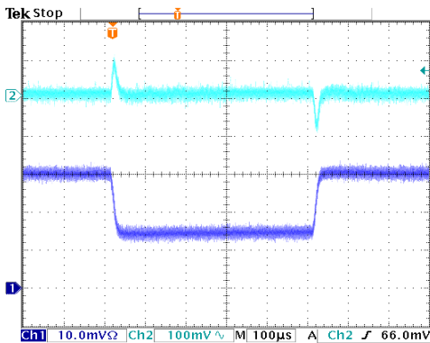
Fig. 14: Load Transient Response CH1:Iout (1A/div) CH2: Vout (3.3V)
