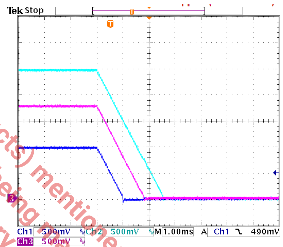
Fig. 13: CH1: 1.0V CH2: 5V CH3: 1.8V Simultaneous Soft-Stop
