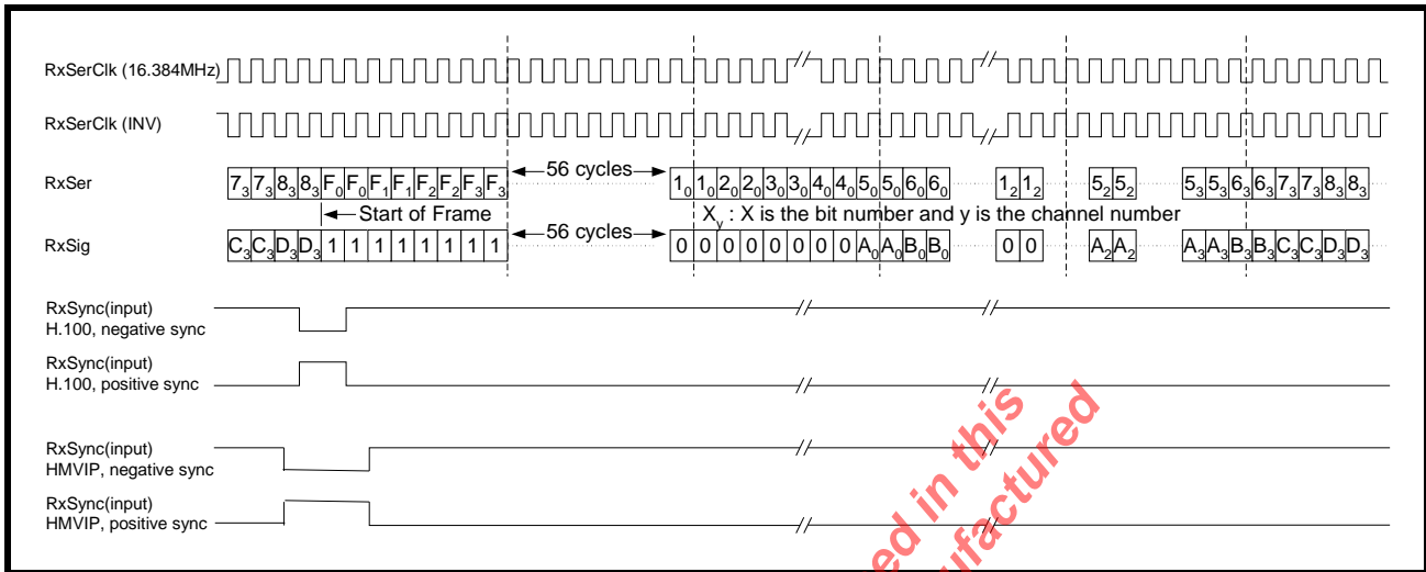
FIGURE 92. WAVEFORMS FOR CONNECTING THE RECEIVE MULTIPLEXED HIGH-SPEED INPUT INTERFACE AT H MVP AND H.100 16.384MBIT/S MODE
