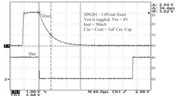
Fig. 27: Turn off time, I_o=50\text{mA} , 4V_{IN}
