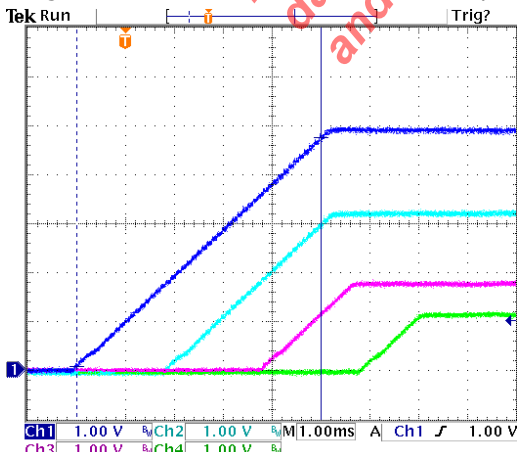
Figure 9: Sequential Start-up
