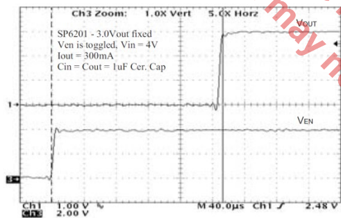
Fig. 24: Turn on time, I_o=300mA , 4V_{IN}
