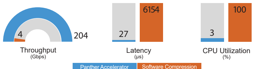
Panther III vs. Software (Direct CPU Core) Compression
