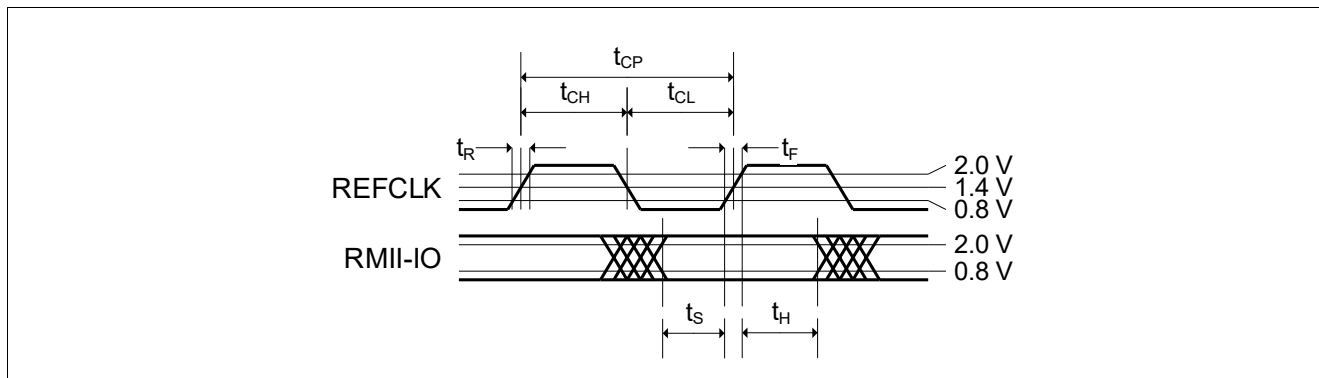
Figure 50 Transmit/Receive Timing Diagram of the RMI
