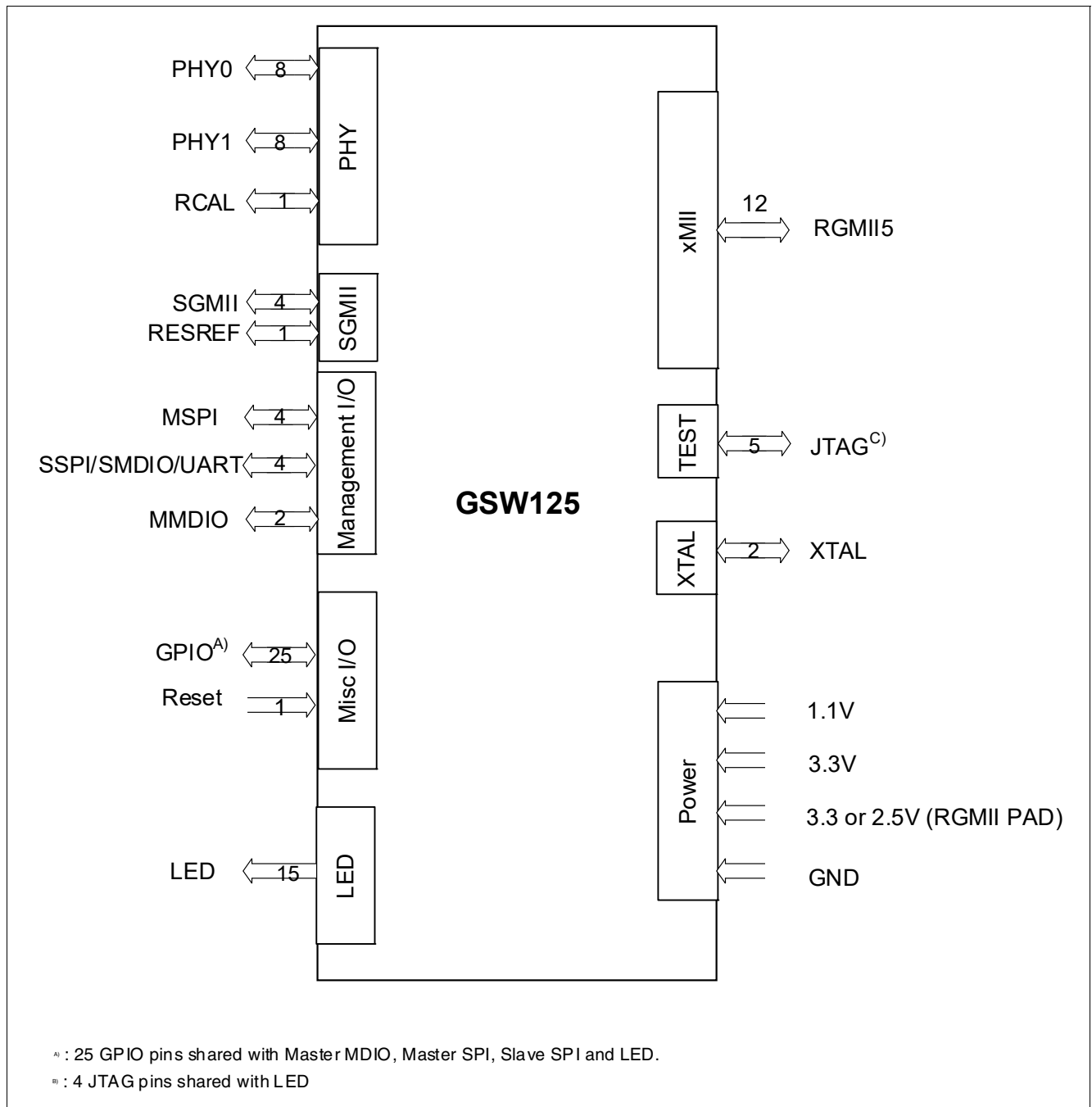
Figure 5 GSW125 Logic Symbol
