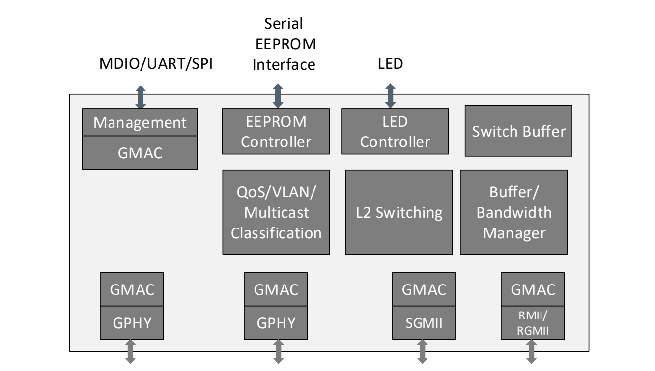
Figure 4 Block Diagram
