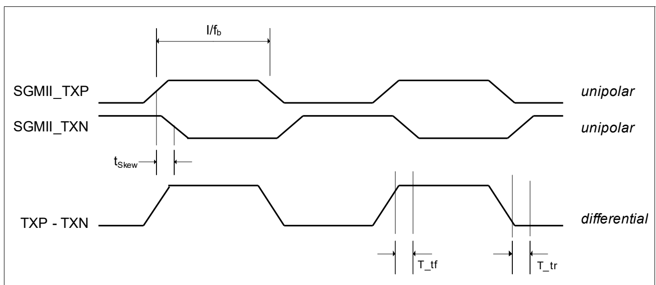
Figure 52 Transmit Timing Diagram of the SGMII (Shows Alternating Data Sequence)
