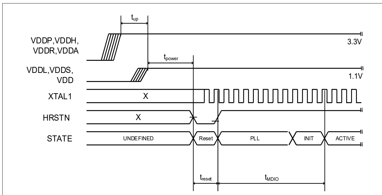
Figure 47 Timing Diagram for the GSW125 Reset Sequence
