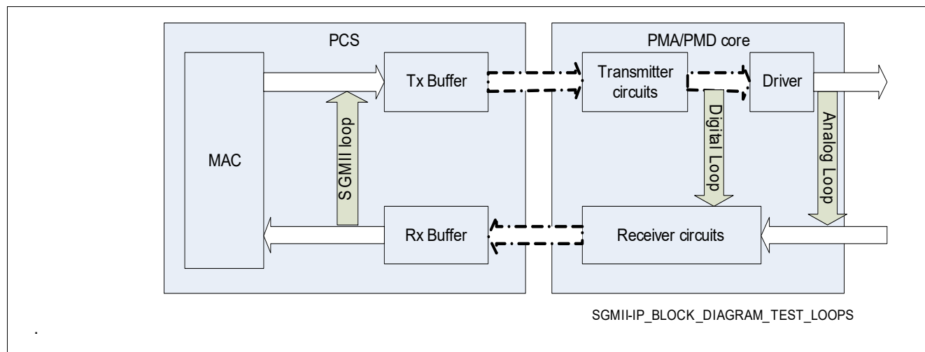
Figure 22 Test Loops in the GSW125
