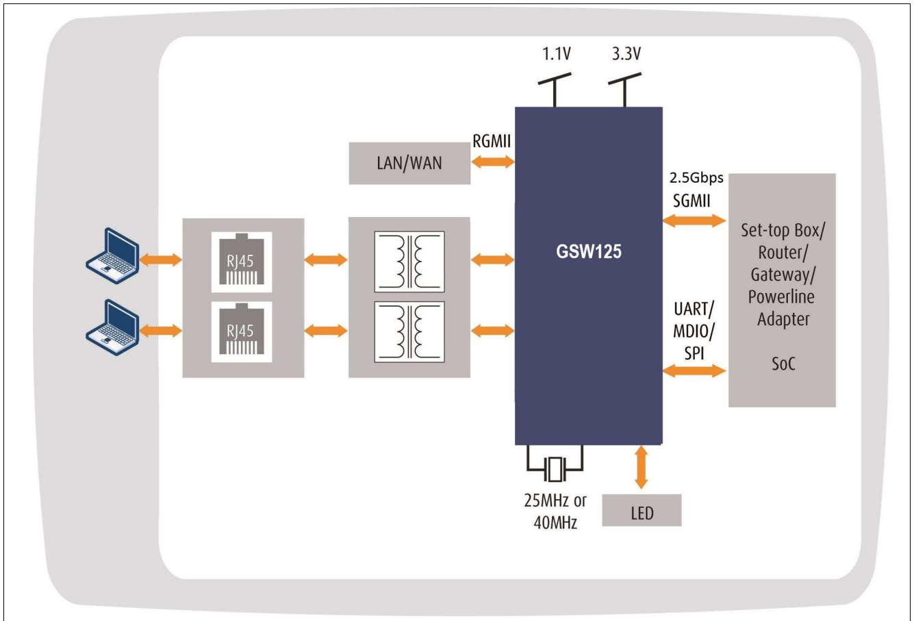
Figure 3 Home Gateway
