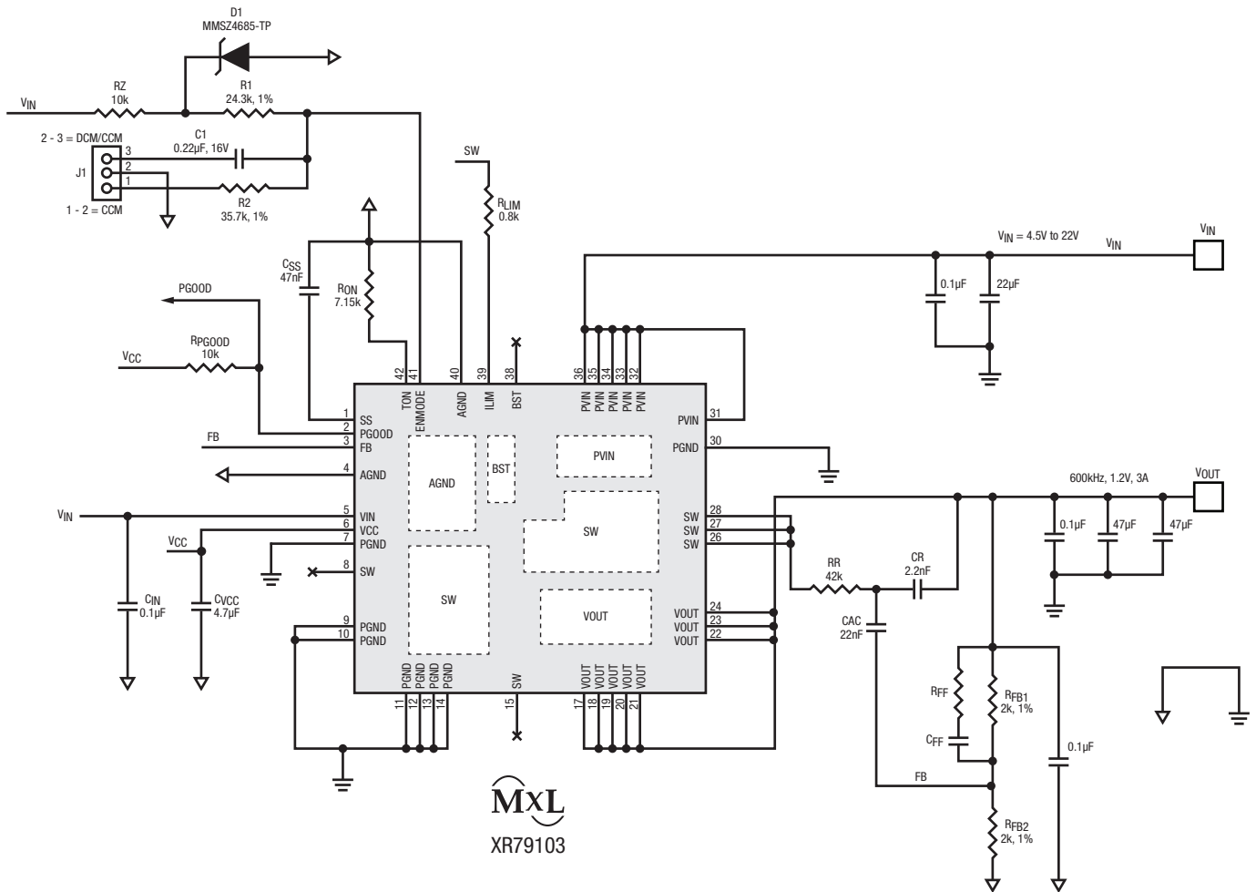
Figure 28. Typical Application Circuit using Alternate Landing Pattern
