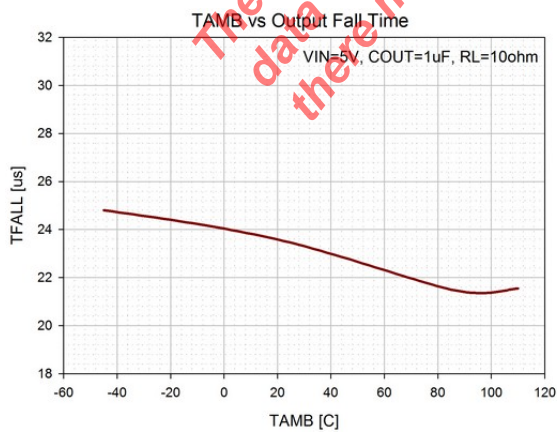
Fig. 14: Output Fall Time vs. Temperature
