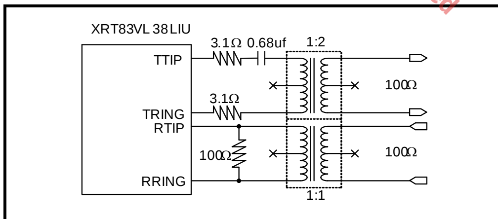
FIGURE 14. SIMPLIFIED DIAGRAM FOR T1 IN THE EXTERNAL TERMINATION MODE (RXTSEL= 0 & TXSEL= 0)
